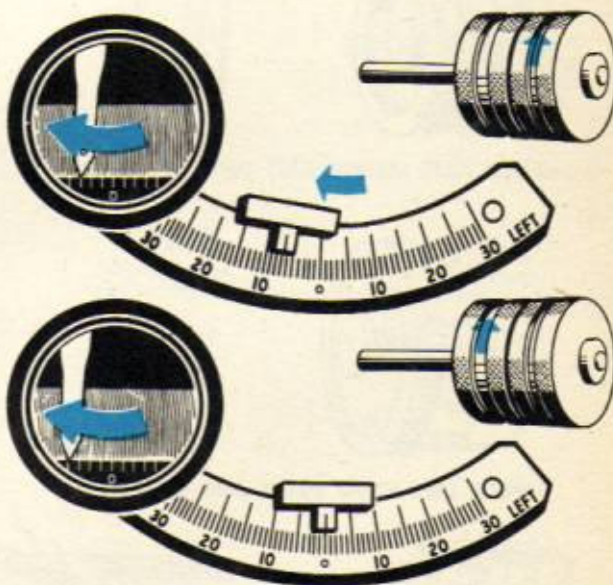
CHECK FOR MIRROR DRIVE CABLE LENGTH
